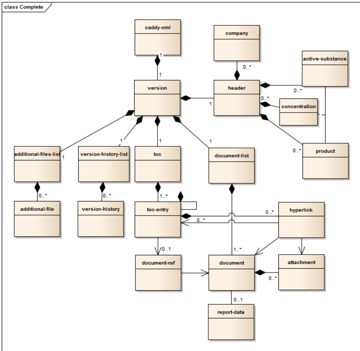
Figure 12: Overview CADDY-xml (v3) Elements
