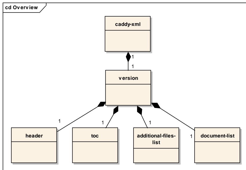
Figure 1: XML-Backbone Overview
