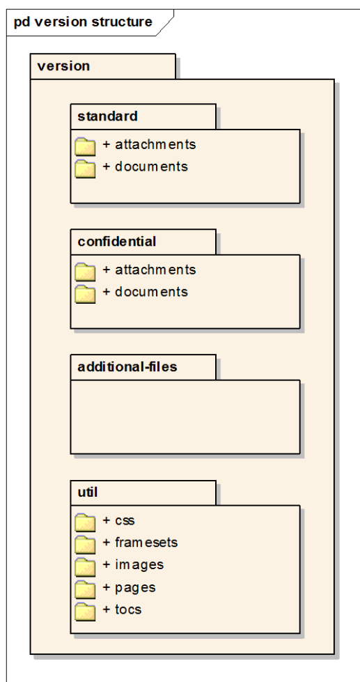
Figure 11: Version Structure
