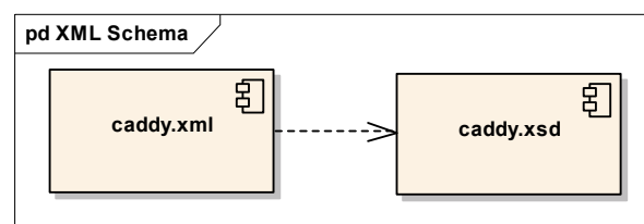
Figure 3: XML Schema
