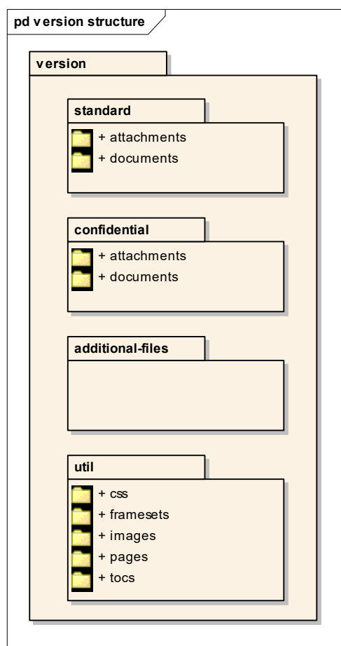
Figure 11: Version Structure
