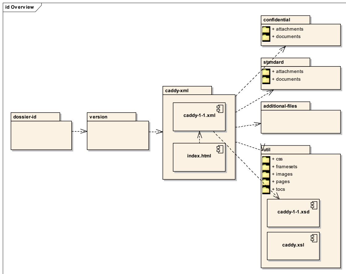
Figure 2: File-System Organization
