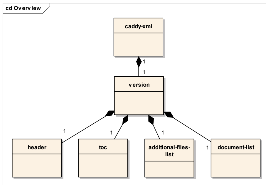
Figure 1: XML-Backbone Overview
