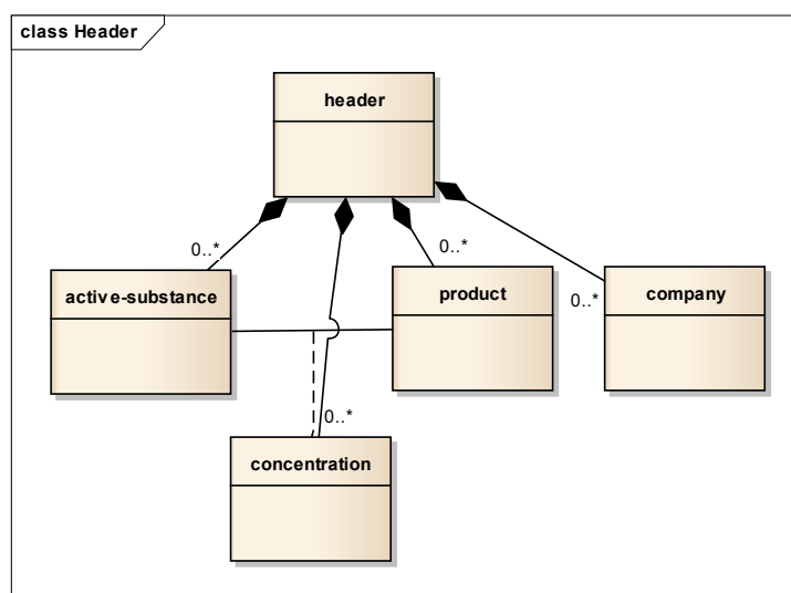
Figure 4: Header
