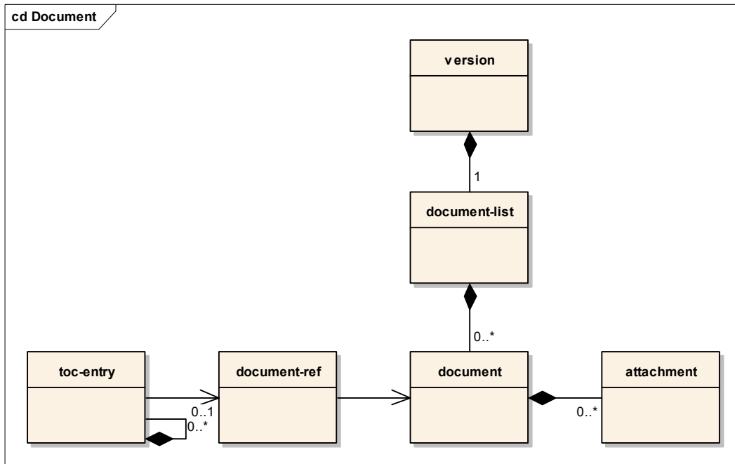
Figure 6: Document List
