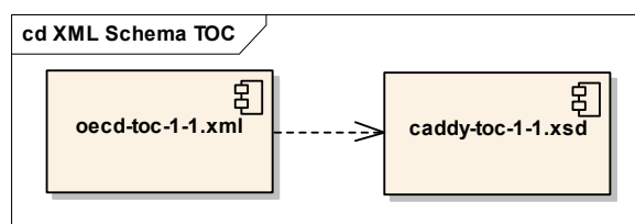
Figure 8: XML Schema
