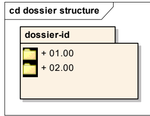
Figure 10: Dossier Structure
