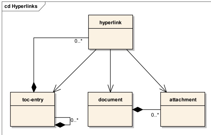
Figure 7: Hyperlinks
