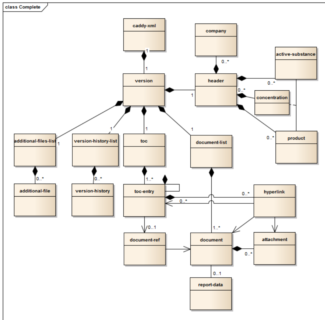
Figure 12: Overview CADDY-xml (v3) Elements
