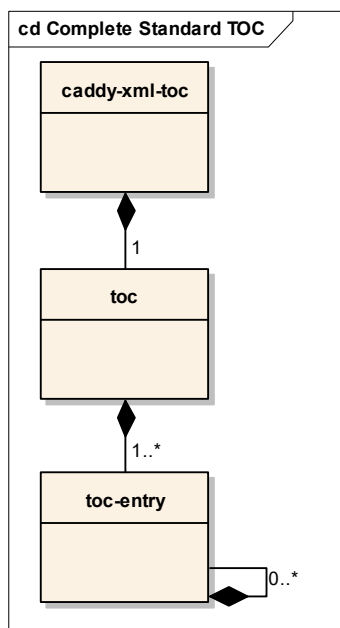
Figure 13: Overview CADDY-xml (v3) Standard TOC Elements
